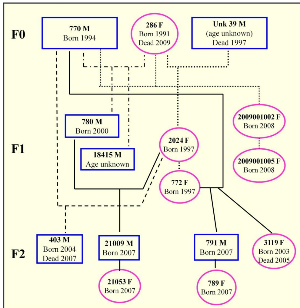
Figure 10. Most likely pedigree resulting from translocated female grizzly bear 286 into the Cabinet Mountains, USA, 1993-2009. Squares indicate males and circles represent females. Lines indicate a parent-offspring relationship. F0 is the initial generation, F1 is the first generation of offspring for translocated female 286, and F2 is the second generation.
