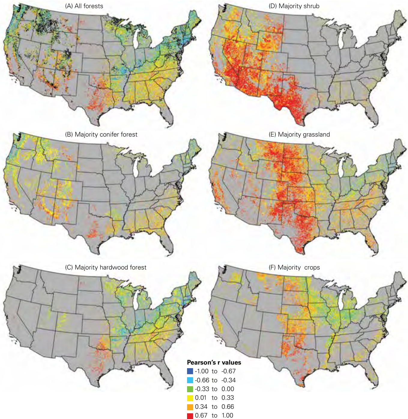
Figure 9.12—Correlations (Pearson's r ) between mean March–September Moderate Resolution Imaging Spectroradiometer (MODIS)-based ForWarn Normalized Difference Vegetation Index (NDVI) and National Land Cover Data Climate Division mean monthly March–September Palmer Modified Drought Index (PMDI) for majority land cover types derived from the NLCD showing areas of known disturbance by wildland fire or biotic insect or disease in black for (A) all forests, (B) majority conifer, (C) majority hardwood, (D) majority shrub, (E) majority grassland, and (F) majority crops, 2000–2012. Wildland fire was derived from http://www.MTBS.gov (2000–2012) and http://www.GeoMac.gov (2013) (accessed September 1, 2014); insect and disease disturbance was compiled from Forest Service Forest Health Protection (FHP) Insect and Disease Survey (IDS) data. Data shown are based on 250,000 random points, sampled with a 1-km buffer.
