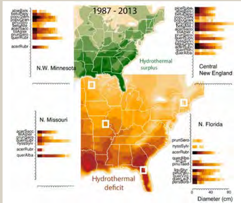
Figure 4.6—Expressed on a relevant scale for trees, such as the number of degree hours at positive (hydrothermal surplus, HTS) and negative (hydrothermal deficit, HTD) water balance, large geographic contrasts contribute to size-species distributions (histograms). Surplus (above) and deficit (below) both reach maximum values near 3000 degree hours, but in different locations. With sufficient moisture, high temperature (up to a point) increases development. Long days and growing seasons combined with moisture (high HTS) benefit species capable of exploiting these conditions in competition with individuals of other species. Conversely, a large number of degree hours at negative water balance benefits species capable of tolerating drought. In the Southeast, surpluses and deficits are both common. The upper Midwest has much lower precipitation, but also lower temperatures and shorter growing seasons. The Northeast benefits from infrequent deficits, despite lower temperatures. Size-species distributions (SSD), shown for four different regions, reflect climate differences and stand history (Clark and others, In press).
