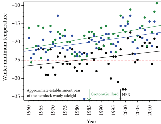
FIGURE 2: Winter minimum temperatures (1960–2013) at Groton, Connecticut (41.35°N, -72.03°W; green symbols), Storrs, Connecticut (41.81°N, -72.25°W; blue symbols), and Harvard Forest (HFR; black symbols) (42.53°N, -72.19°W) along with approximate establishment dates of the hemlock woolly adelgid ( Adelges tsugae ) in southern Connecticut and at Harvard Forest (green and black arrows). Solid lines are best-fit linear temperature trends; the dashed red line at -25°C indicates the LT_{50} for the hemlock woolly adelgid—the temperature at which 50% mortality of the adelgid is expected [46, 47].
