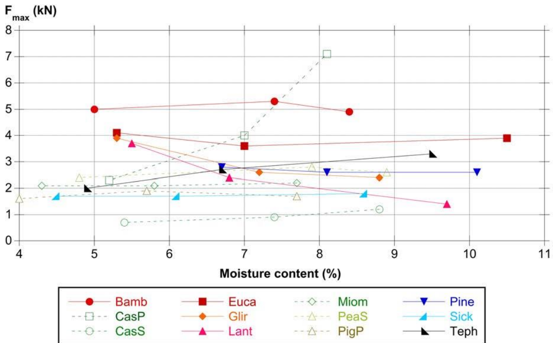
Fig. 3. Maximal backpressure, F_{max} at different MCs, for all tested materials. The lines between the dots do not describe the regression or the inclination, the lines should be seen as help for the reader to follow the materials trends.
