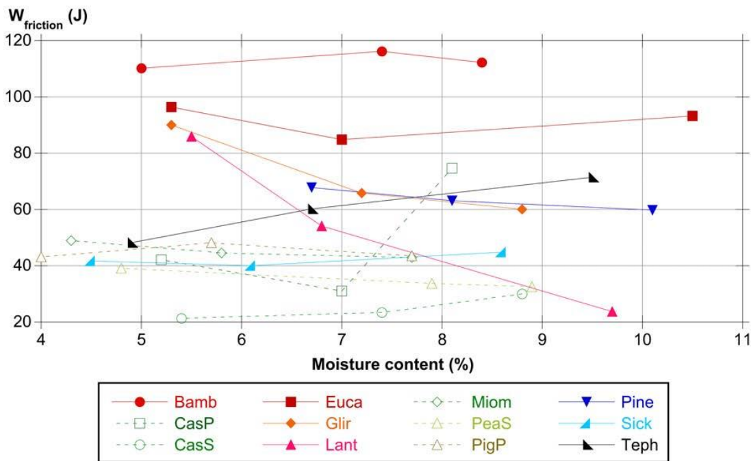
Fig. 4. Friction work, W_{\text{fric}} for all materials at different MCs. The lines between the dots do not describe the regression or the inclination, the lines should be seen as help for the reader to follow the materials trends.
