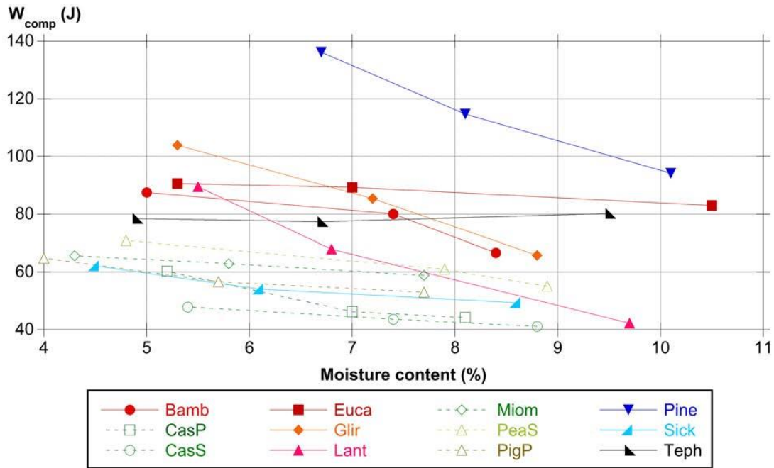
Fig. 2. Compression work, W_{comp} from 1 kN to 14 kN for all tested materials at different MC. The lines between the dots do not describe the regression or the inclination, the lines should be seen as help for the reader to follow the materials trends.
